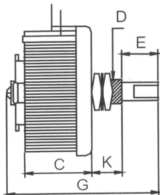
Variable Resistors Side View (FVR) Dimensions
