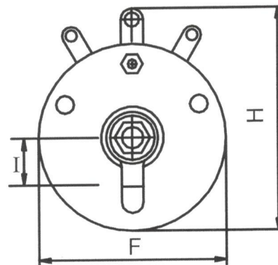
Variable Resistors Bottom View (FVR) Dimensions
