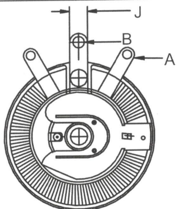
Variable Resistors Top View (FVR) Dimensions
